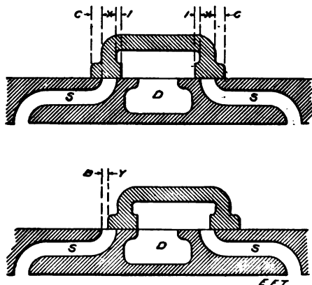
FIG. 236.—Diagrams illustrating the "Lap" and "Lead" of a Steam Cylinder Slide Valve. In both sections, S and S are the steam ports, and D the exhaust. The upper section illustrates the "laps" of a valve; the space between the lines C and X giving the "outside lap," and between the lines X and I the "inside lap." The lower section illustrates the "lead" of a valve; the space between lines B and Y showing the opening of the valve at the beginning of the right-hand stroke.
